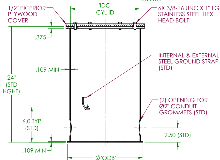
SECTION A-A WITH PLYWOOD COVER AND MACHINE SCREWS
