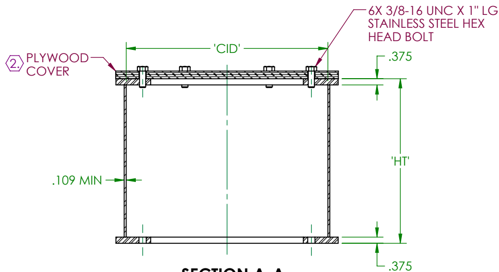
SECTION A-A WITH PLYWOOD COVER AND MACHINE SCREWS
